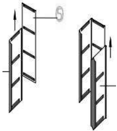
Step1: Install the left side and back panel and middle side
