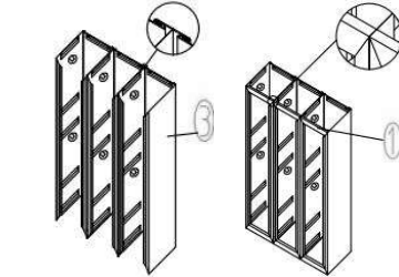
Step4: Install right side and front frame
