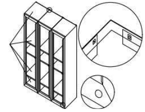
Step6: Install top plate and shelves
