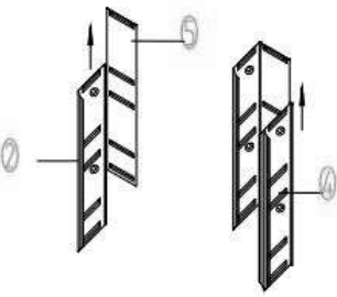
Step1: Install the left and middle side with back panel
