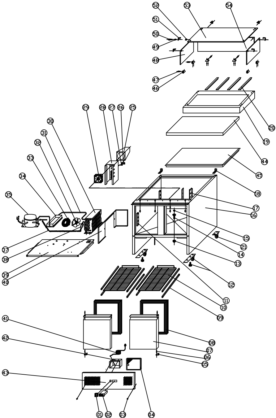
EXPLODE OF G-PS200G
