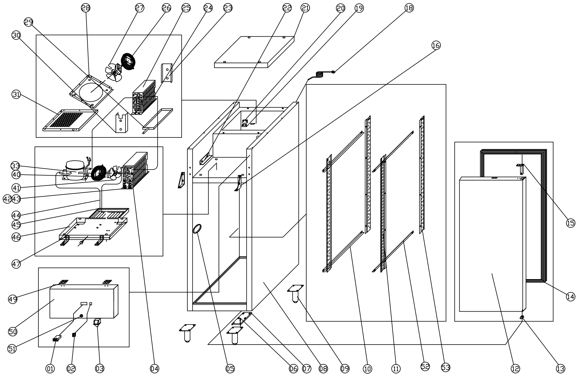
EXPLODE DIAGRAM OF G-PA800TN
