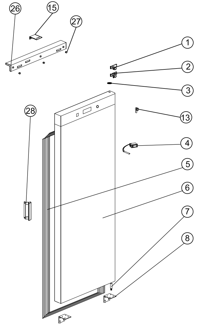
EXPLODE OF G-HT400F
