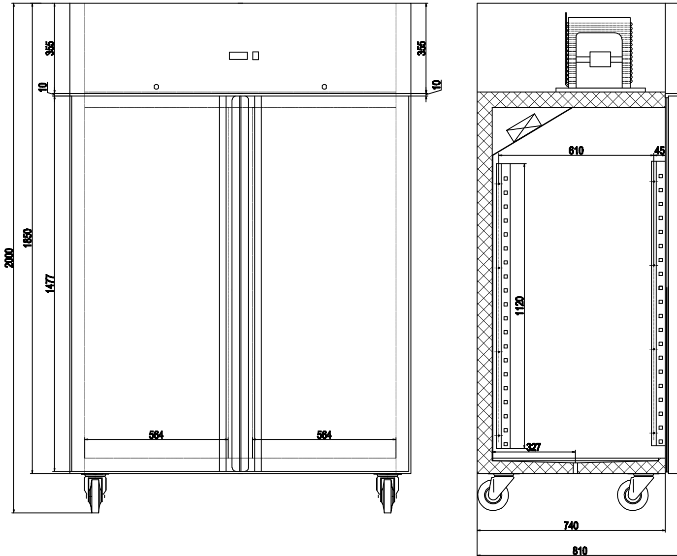
OUTSIDE DRAWING OF G-ECS1200TN
