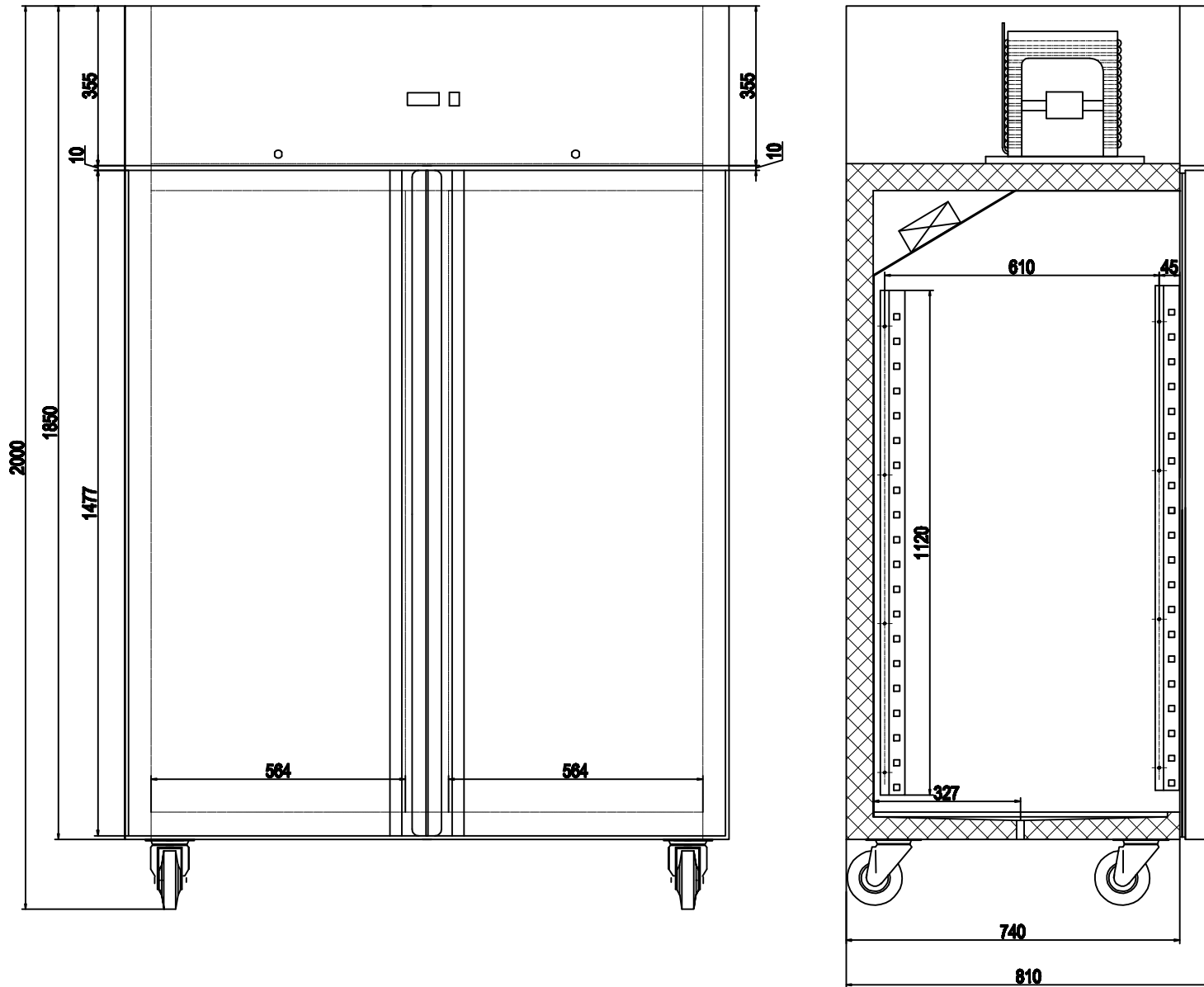
OUTSIDE DRAWING OF ECS1200BT
